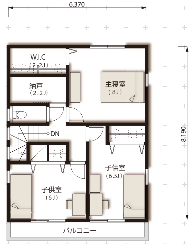
2nd floor
