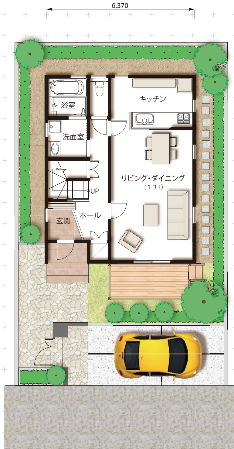
1st floor
